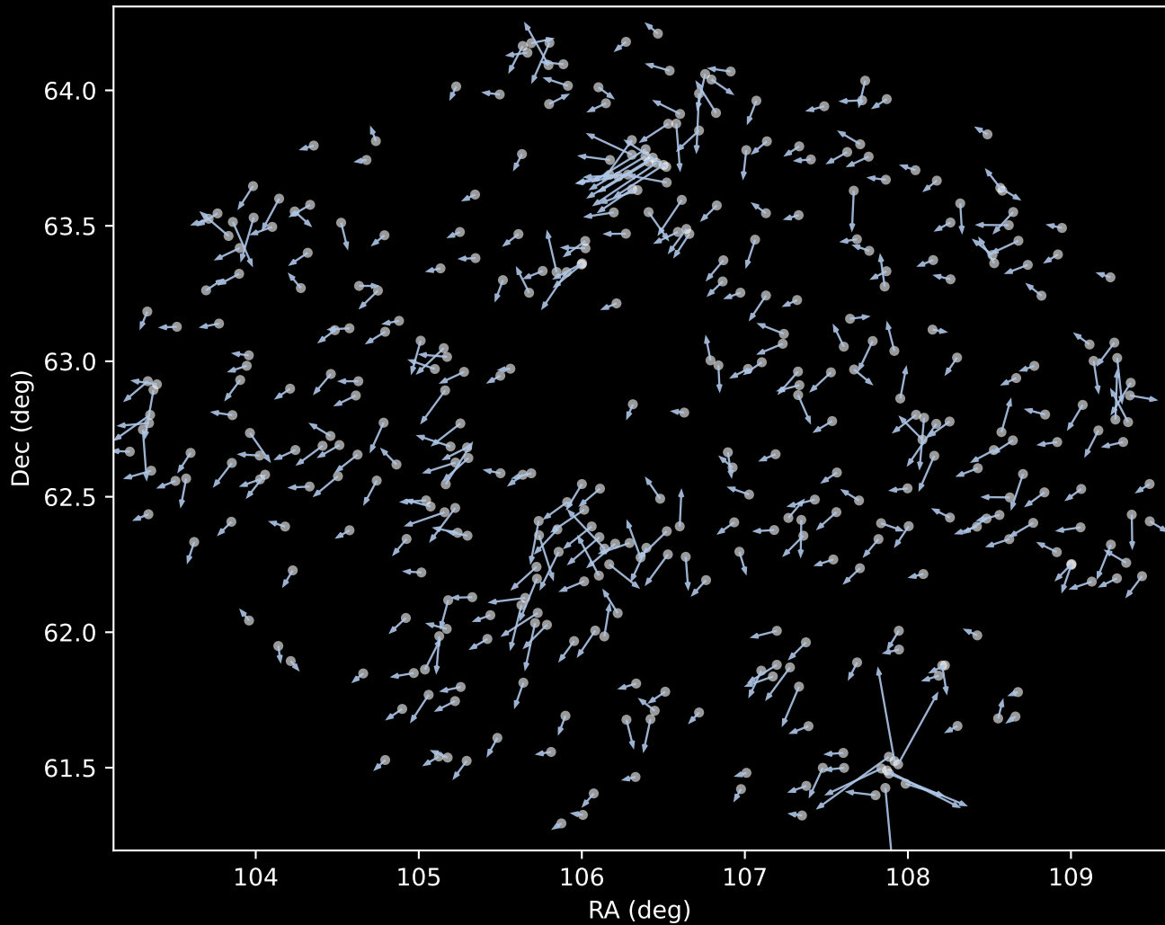
APOGEE DR17 Cluster 1 Proper Motion Vectors (n=397)
