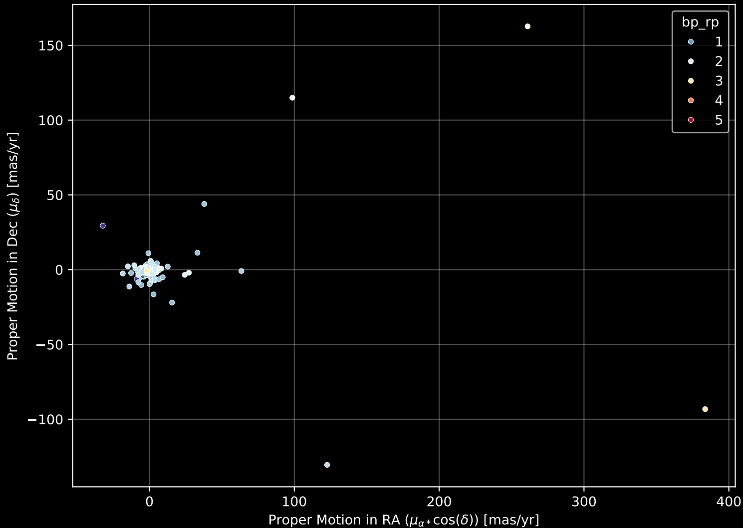
APOGEE DR17 Field: [120+00] Proper Motion Diagram (n= 440)
