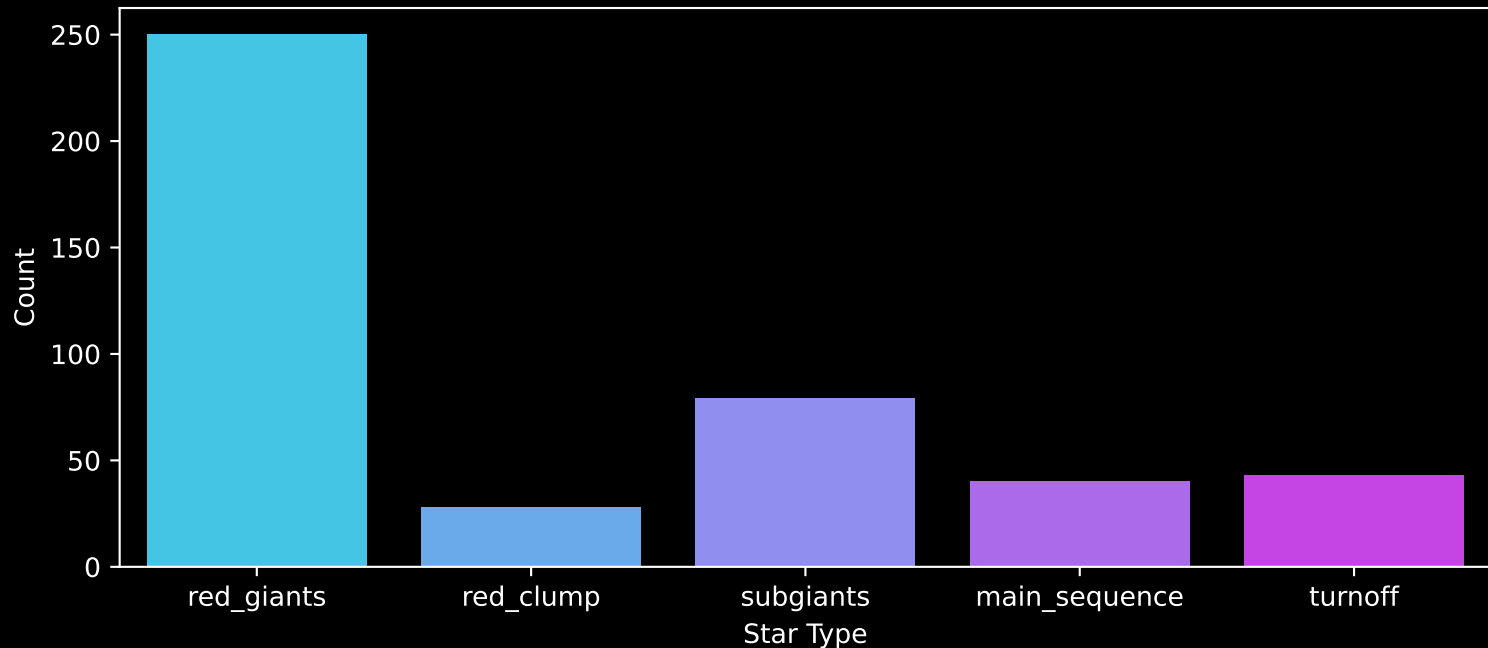
APOGEE DR17 Field: [120+00] Count plot of Star Type
