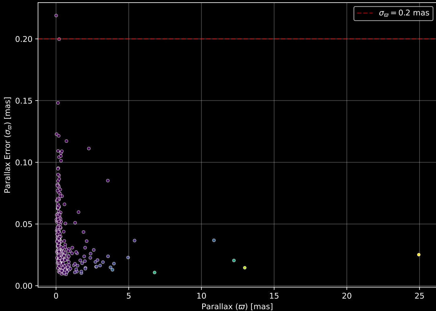
APOGEE DR17 Field: [120+00] Parallax Quality (n= 440)
