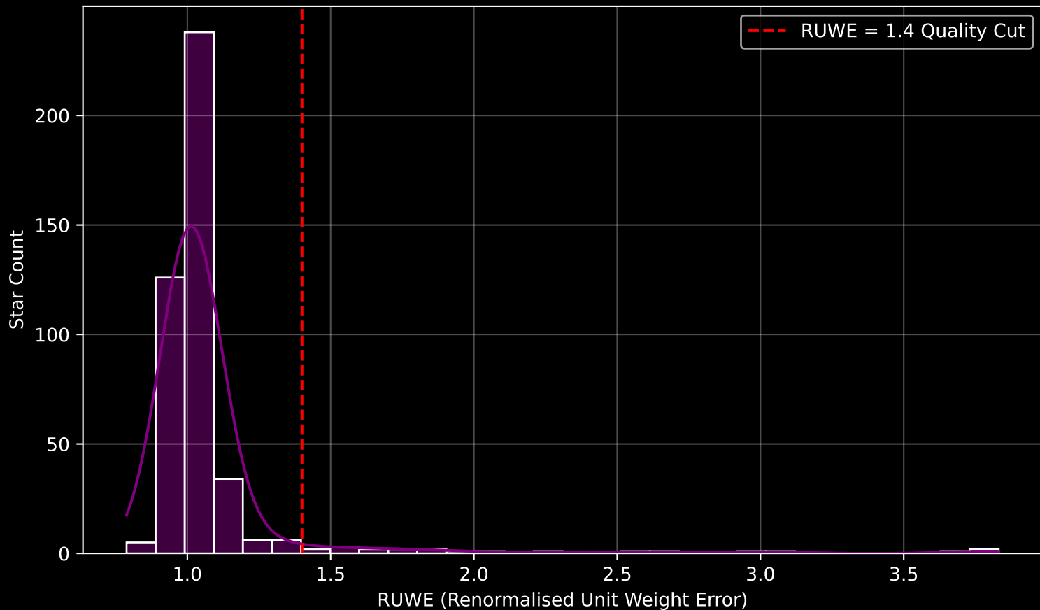
GAPOGEE DR17 Field [120+00] RUWE Distribution (n= 436)
